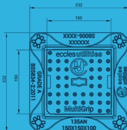
B-B (1:8)
